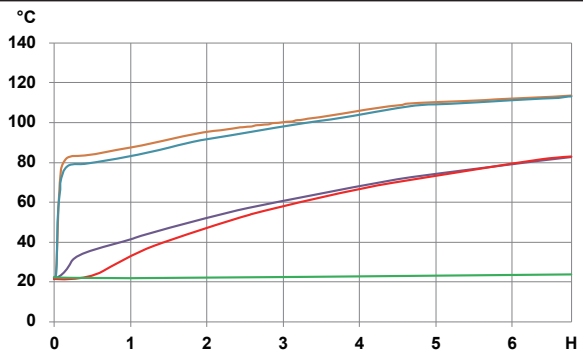
Variation in the temperature versus time of a 220-liter metal drum, filled with HF 24-6 hydraulic oil, heated by a silicone heating belt 200mm wide, without thermal insulation, power 1500W (surface power load 0.5W/cm 2 ).
